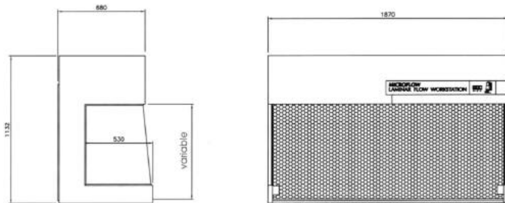
1.8m workstation
